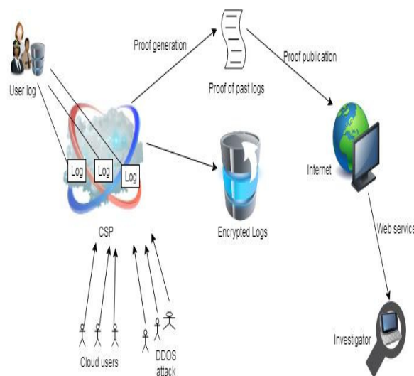
Fig. 1 Proposed DDoS Framework
