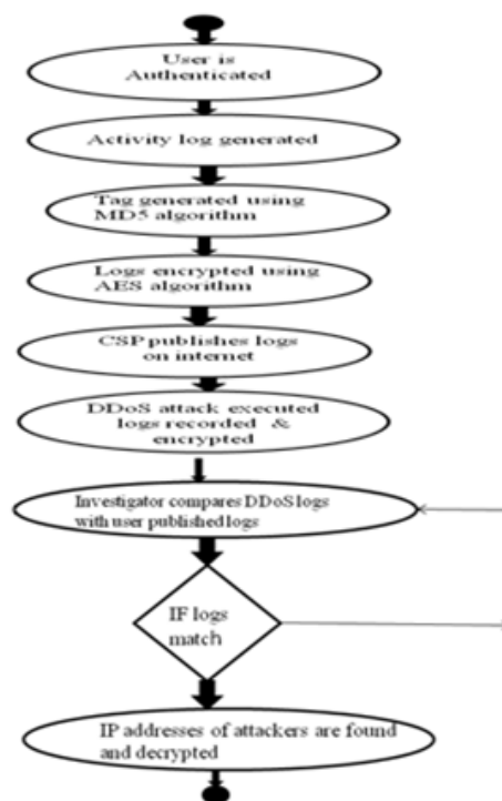
Fig. 2 Flowchart DDoS System
